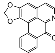
6. Liriodenine
