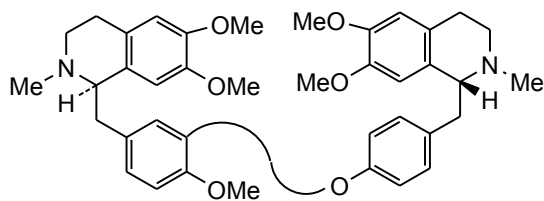
10. Dauricine-O-methyl ether
