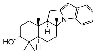
14. 3-greenwayodendrinol
