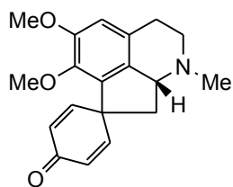
7. Pronuciferine
