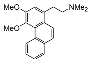
8. Atherosperminine
