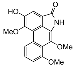
2. Enterocarpam I
