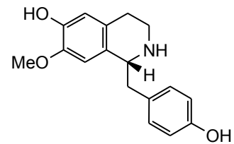
3. Coclaurine
