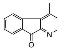
11. Onychine
